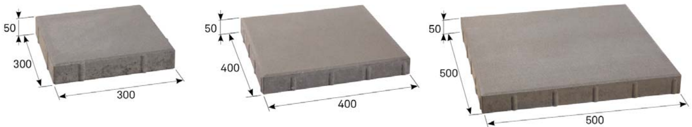
Layout dimensions
