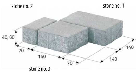
Layout dimensions, set of 3 types of stones
